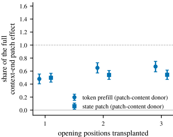
Qwen2.5-7B, format cells
