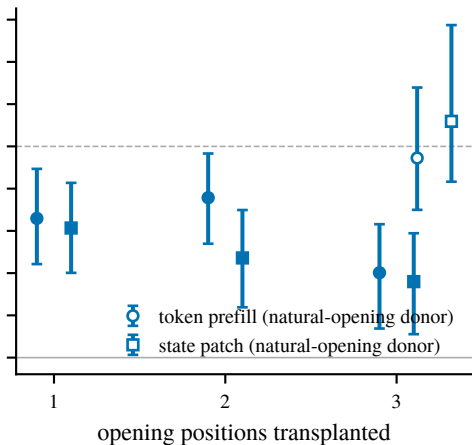
Qwen3.5-9B, language cells (null-adjusted)
