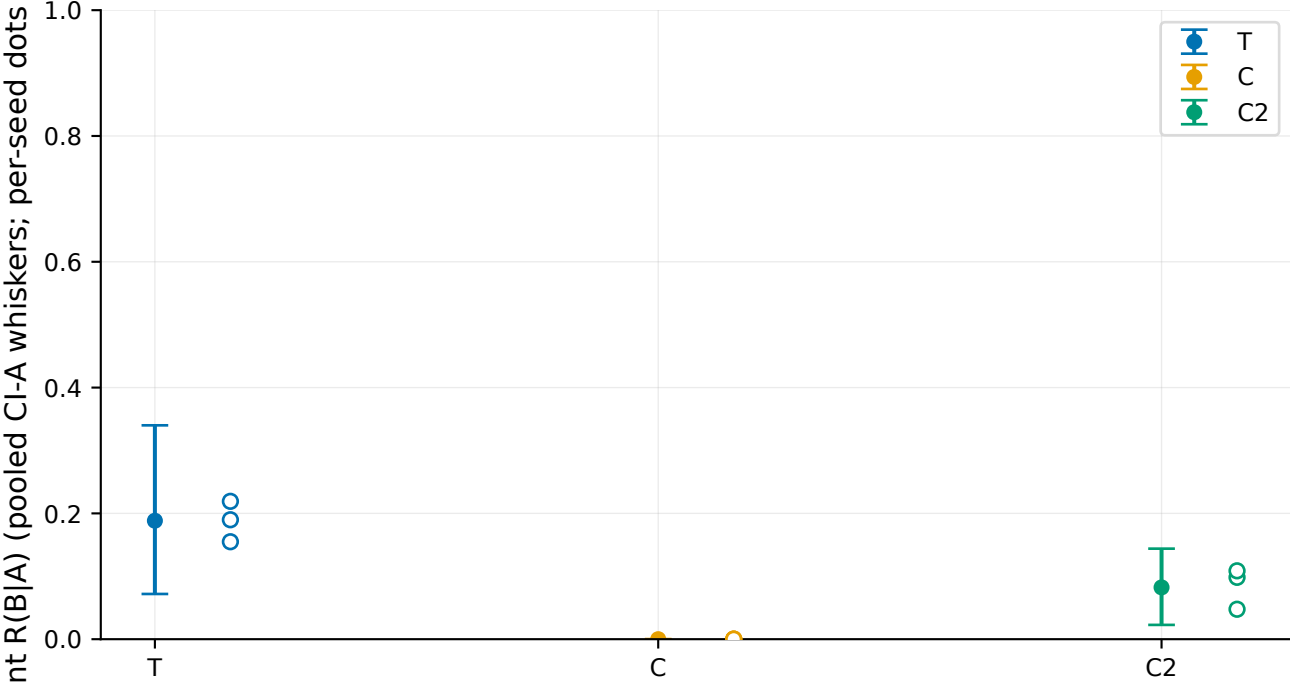
Seed disagreement vs pooled CI per arm
