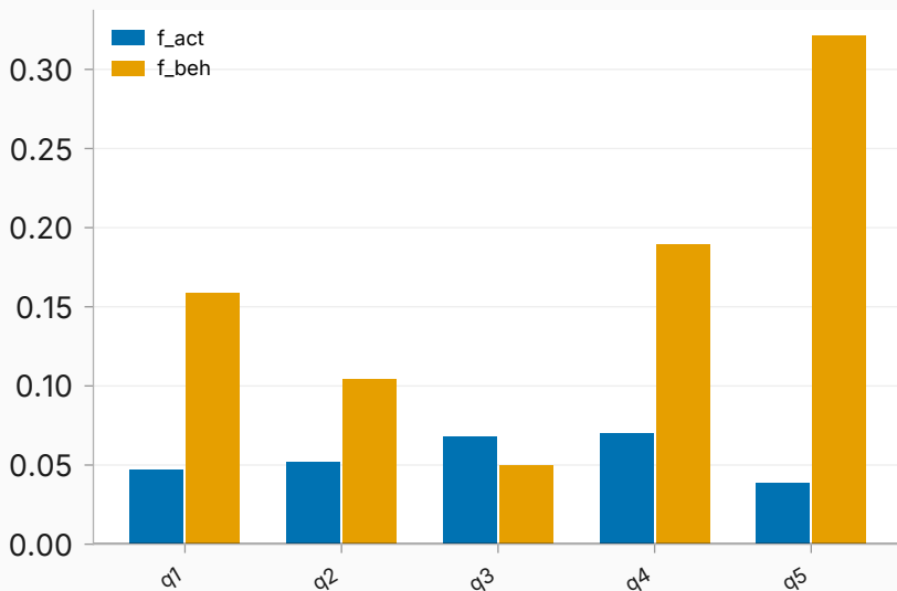
mean F by target query
