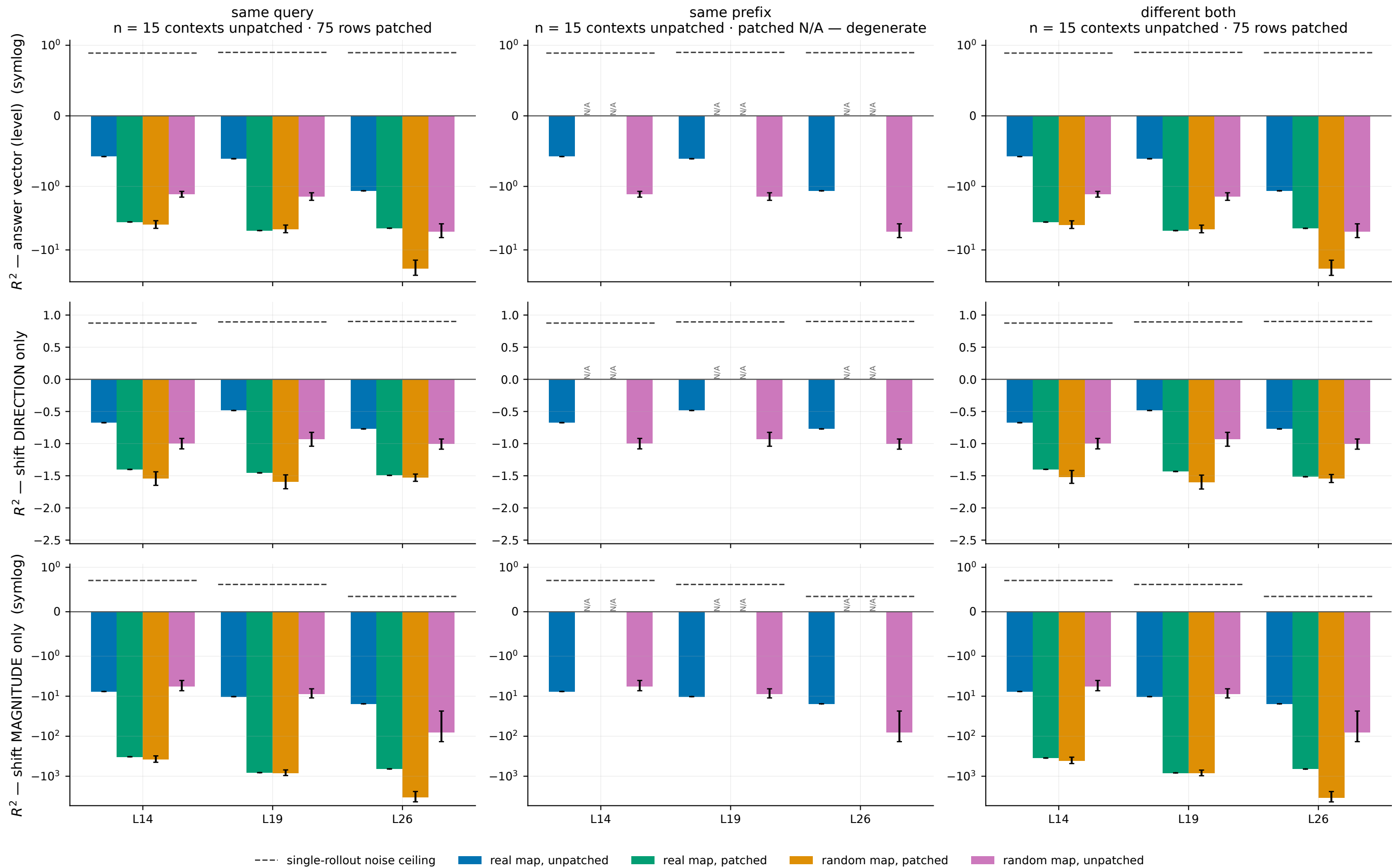
Banked-map R^2 at the prefix-end state: real vs spectrum-matched random map, unpatched vs patched
