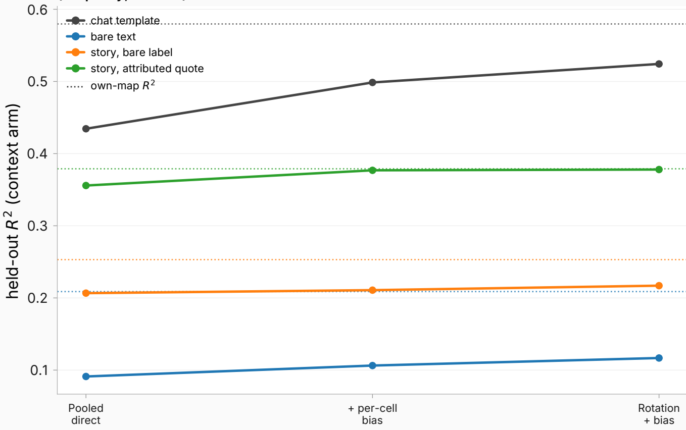
One map fit on all settings, applied to each framing (on-policy, instruct)
