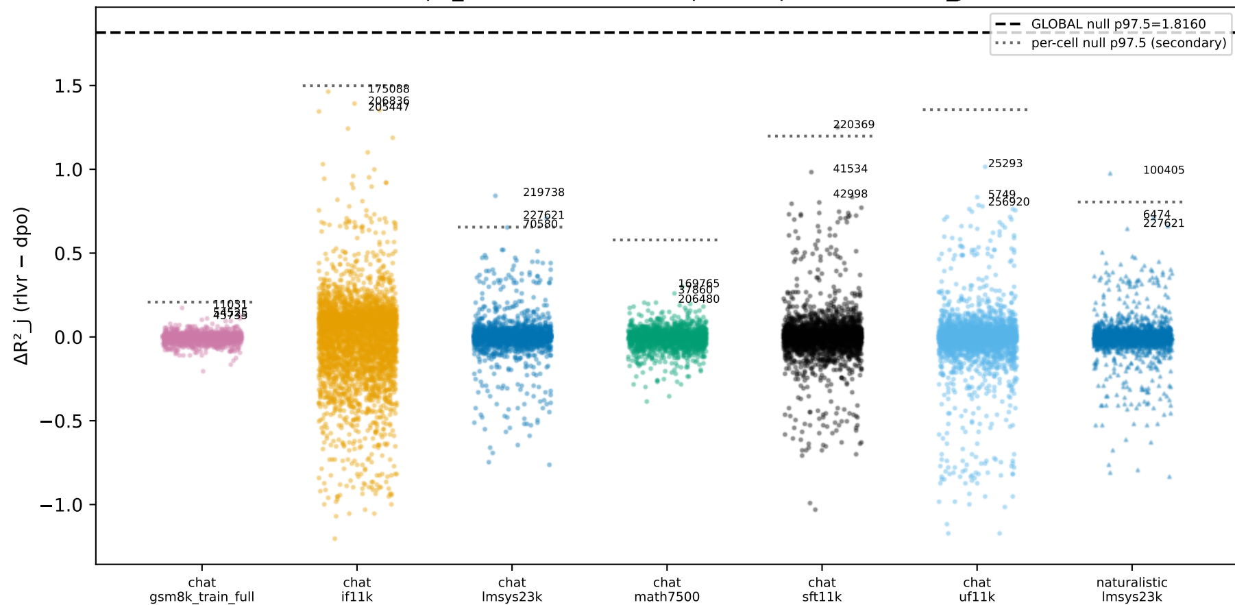
F2: dpo_rlv / context arm — per-cell per-feature \Delta R^2_j
