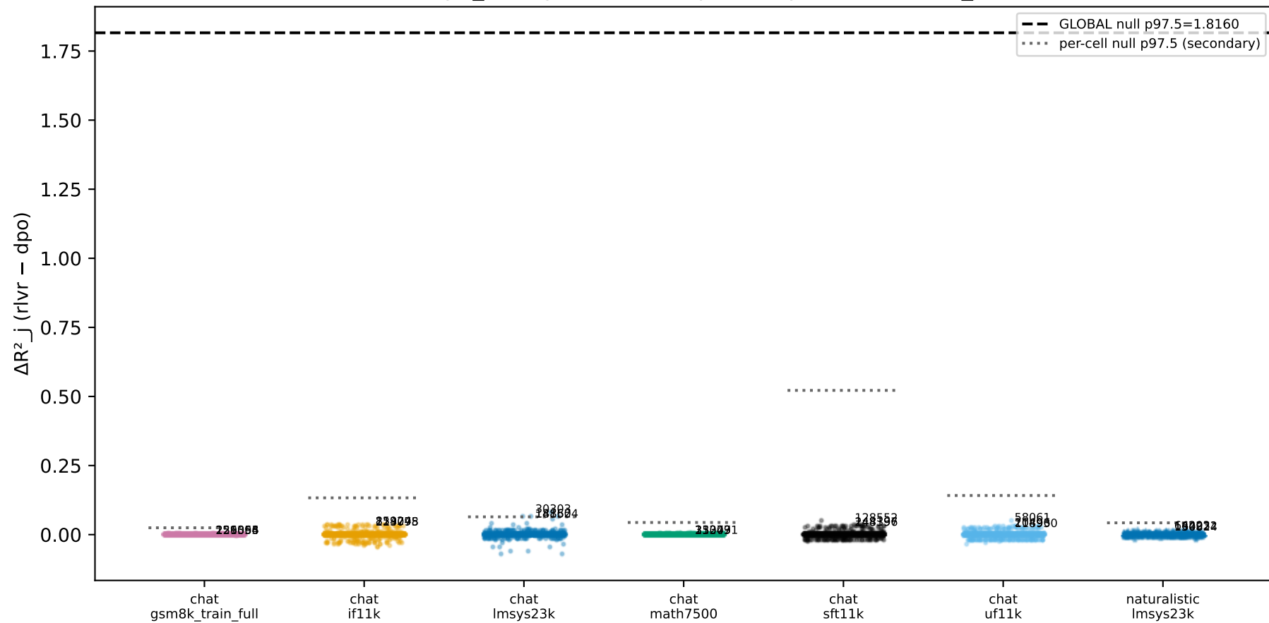
F2: dpo_rlv_r / prefix arm — per-cell per-feature \Delta R^2_j
