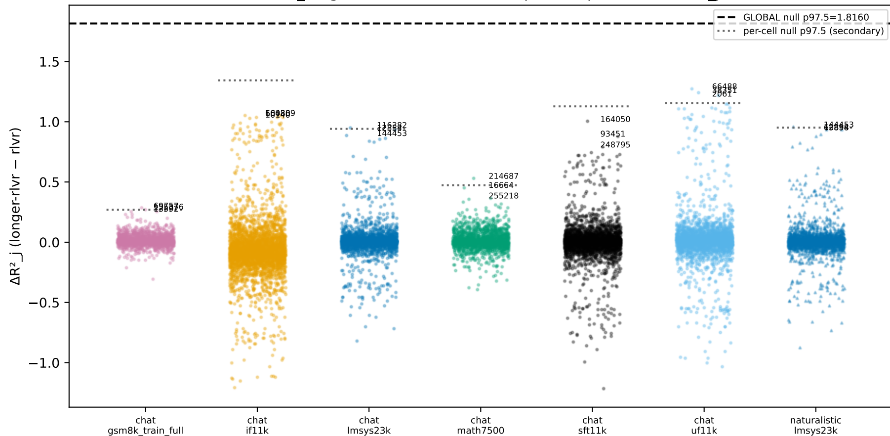
F2: rlvr_longer-rlvr / context arm — per-cell per-feature \Delta R^2_j
