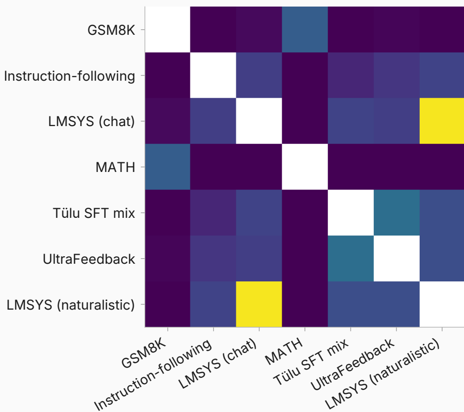
base → SFT
