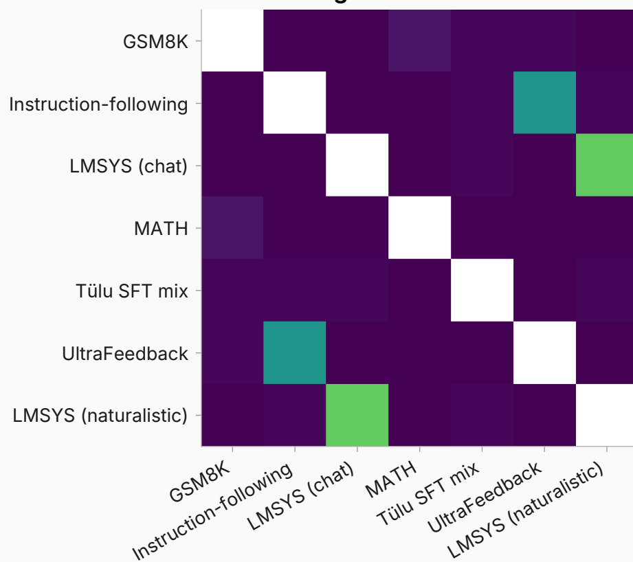
RLVR → longer-RLVR
