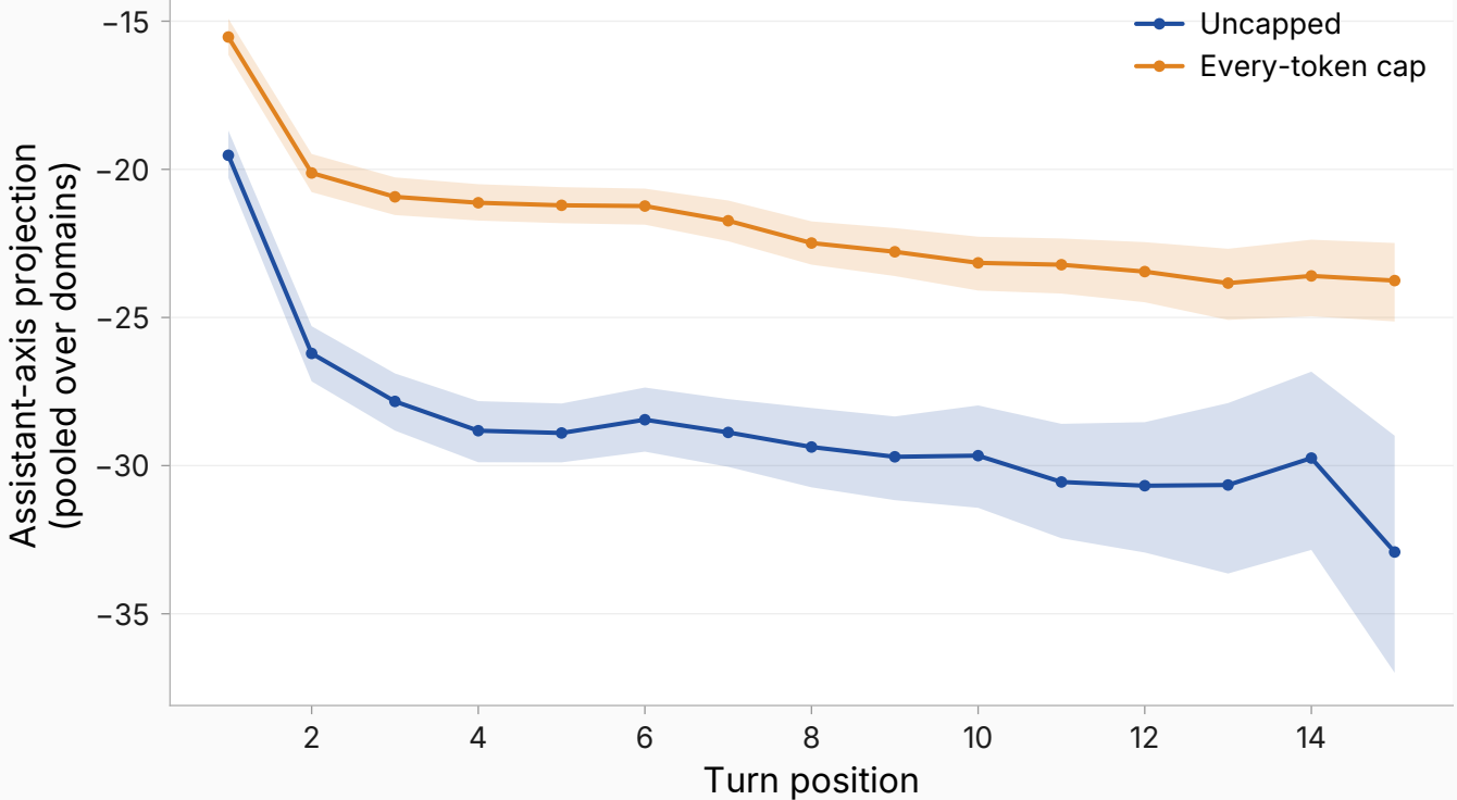
Qwen3-32B drift: uncapped vs every-token cap
