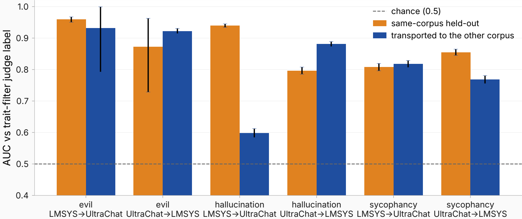
Trait-probe ranking accuracy: train corpus vs the other corpus
