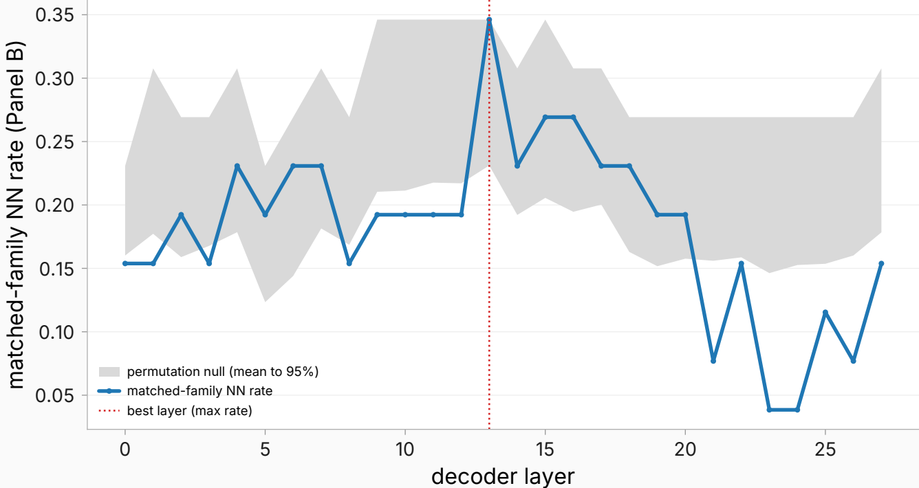
H1: behavior -> nearest-context family match vs depth
