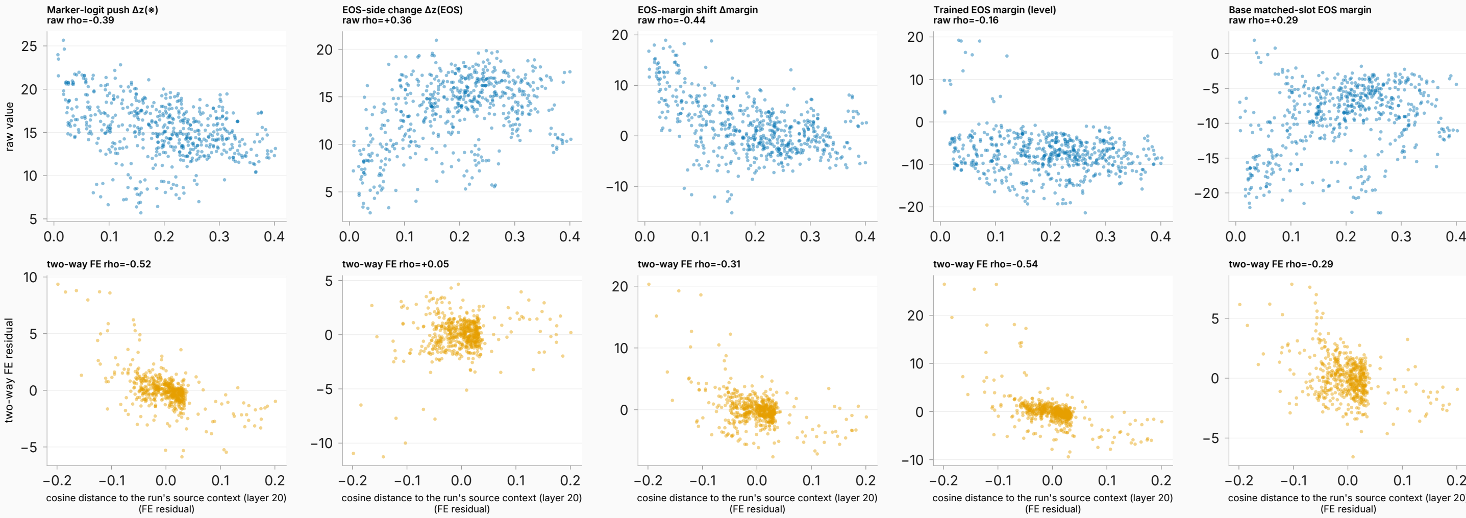
#560 min_dist reads: raw (top) alongside two-way-FE-corrected (bottom)
