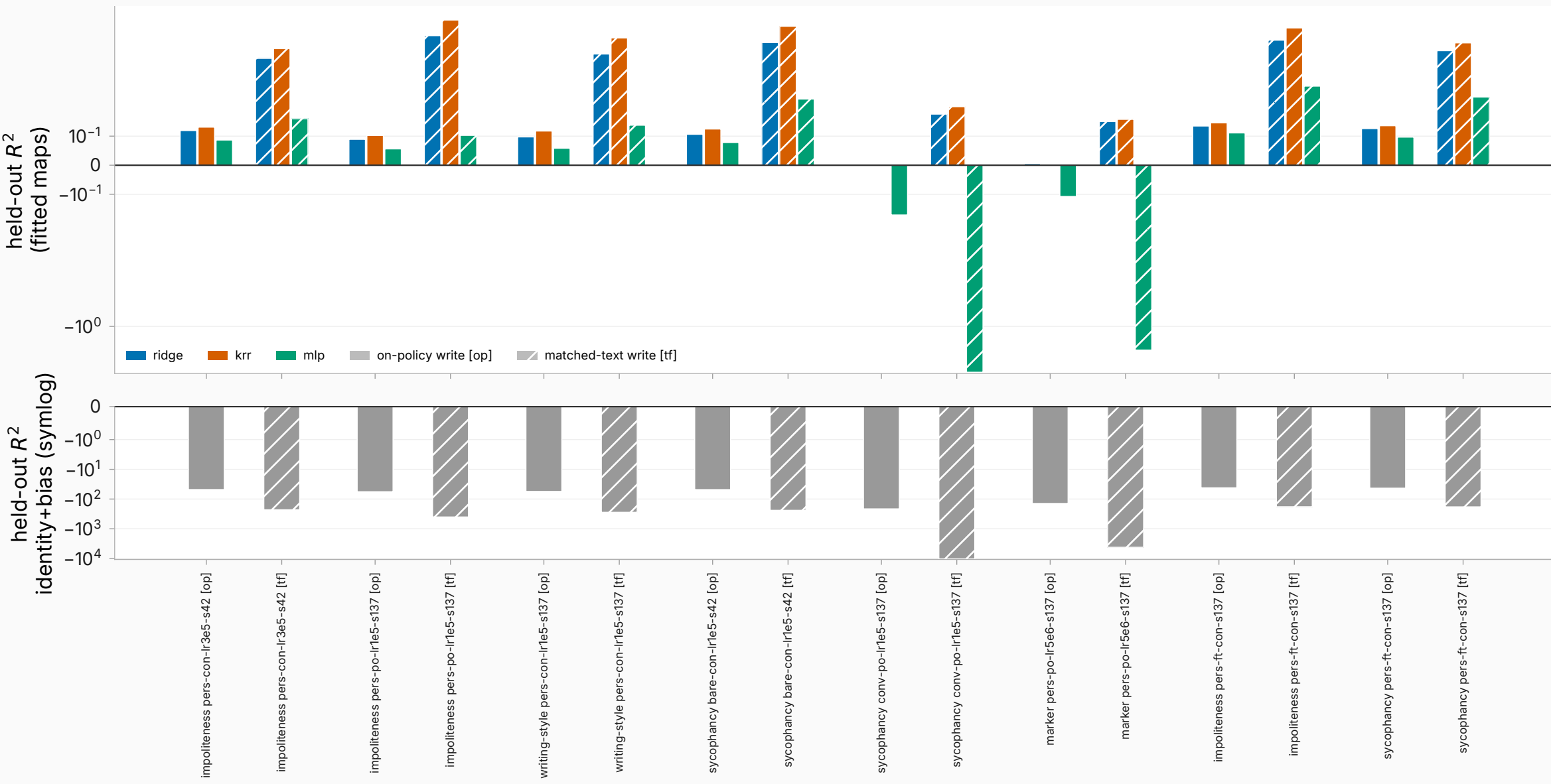
Predicting the per-context write w(x) from the base context vector c_0(x) — layer 19. Variance-weighted R^2 vs the test mean of w , so R^2 > 0 is context-dependent predictability beyond the static mean write.
