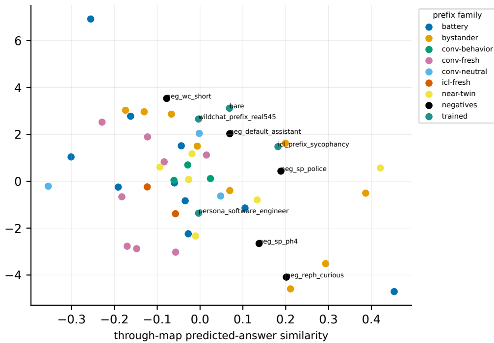
sycophancy bare-context contrastive rho = -0.32, p = 0.0249 (n = 50 prefixes)
