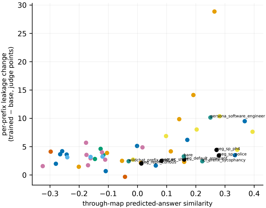
impolite persona contrastive (seed 42) rho = +0.42, p = 0.00271 (n = 50 prefixes)
