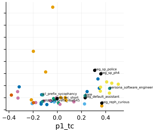
imp-pers-po-lr1e5-s42: per-prefix DV vs {P7, P1, P2} (points = prefixes)
