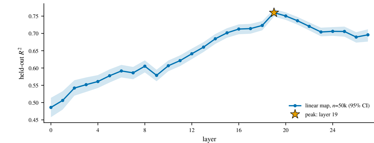
Figure 3. Held-out R^2 against the layer at which both v_C and v_A are taken (swept together). Band: bootstrap 95% CI over test rows. Star: argmax, layer 19 19 and 20 overlap. n_{\text{train}} = 50,000 , n_{\text{test}} = 1,000 .
