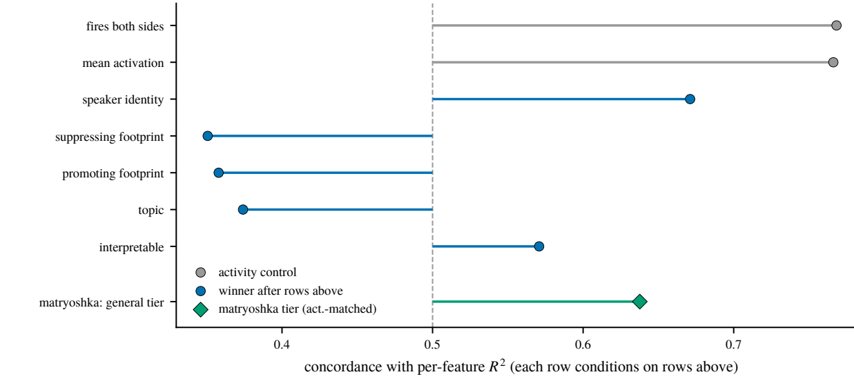
Figure 5. Forward-stepwise partialling: each row conditions on all rows above. c = concordance (AUROC scale), 0.5 = chance. Gray: activity controls. Diamond: matryoshka general tier different dictionary, direction only. No CIs; rounds 7–13 omitted.
