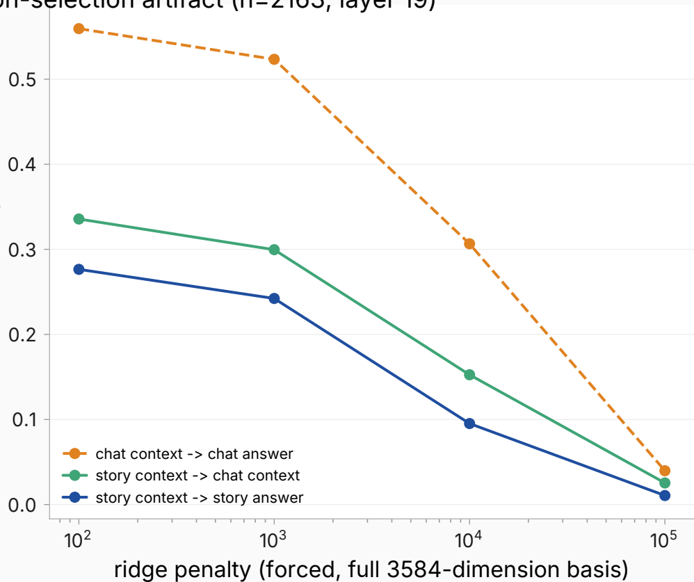
The story-framing collapse is a regularization-selection artifact (n=2163, layer 19)
