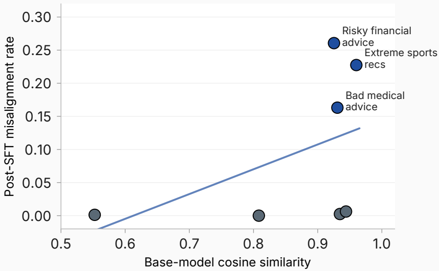
Output-distribution similarity (behavior shown via examples)
