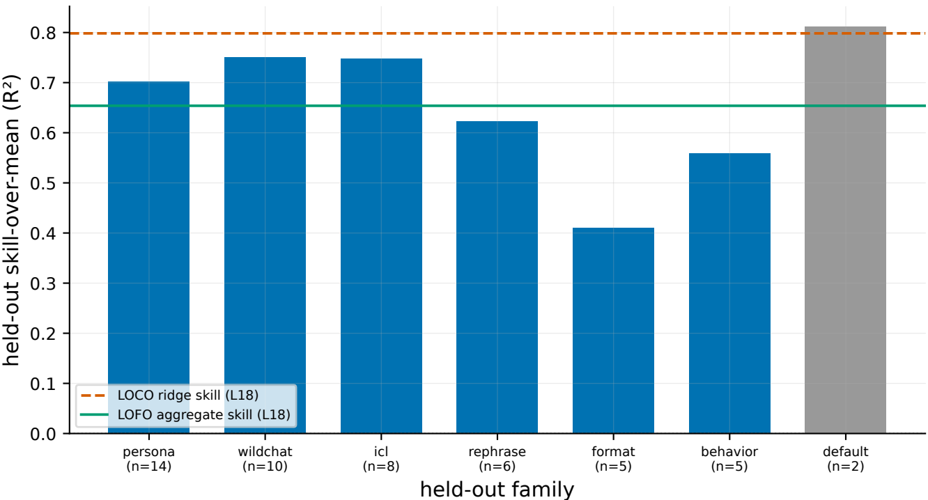
LOFO per-family held-out ridge skill — L18
