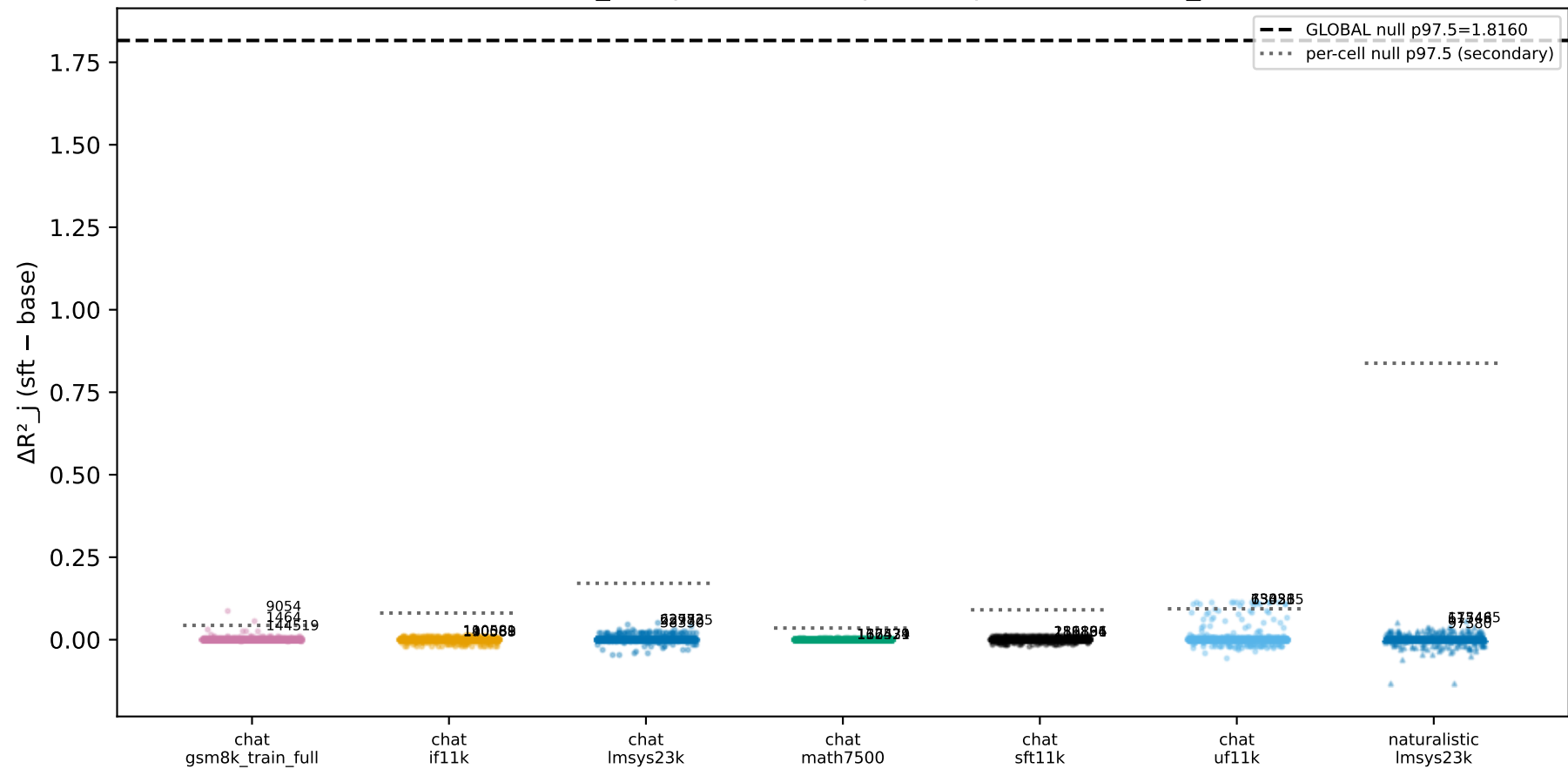
F2: base_sft / prefix arm — per-cell per-feature \Delta R^2_j
