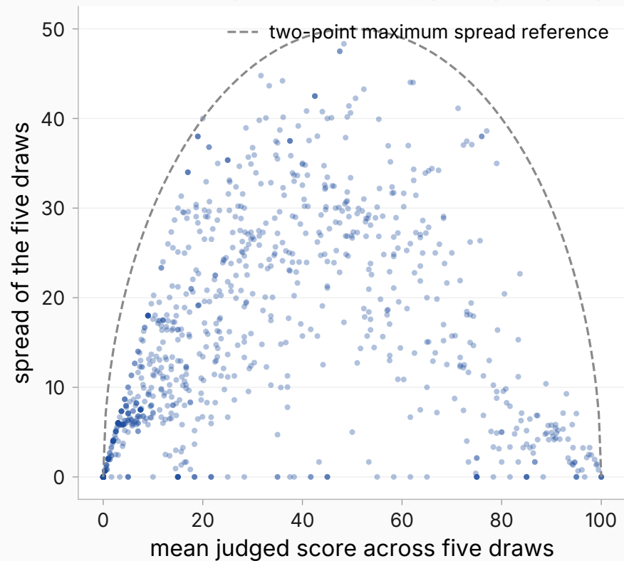
Harmful compliance, training prompts: per-prompt cloud
