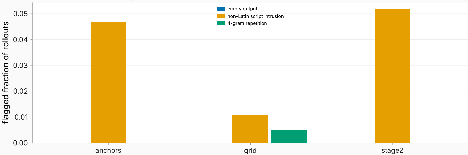
Mechanical audit rates per rollout source
