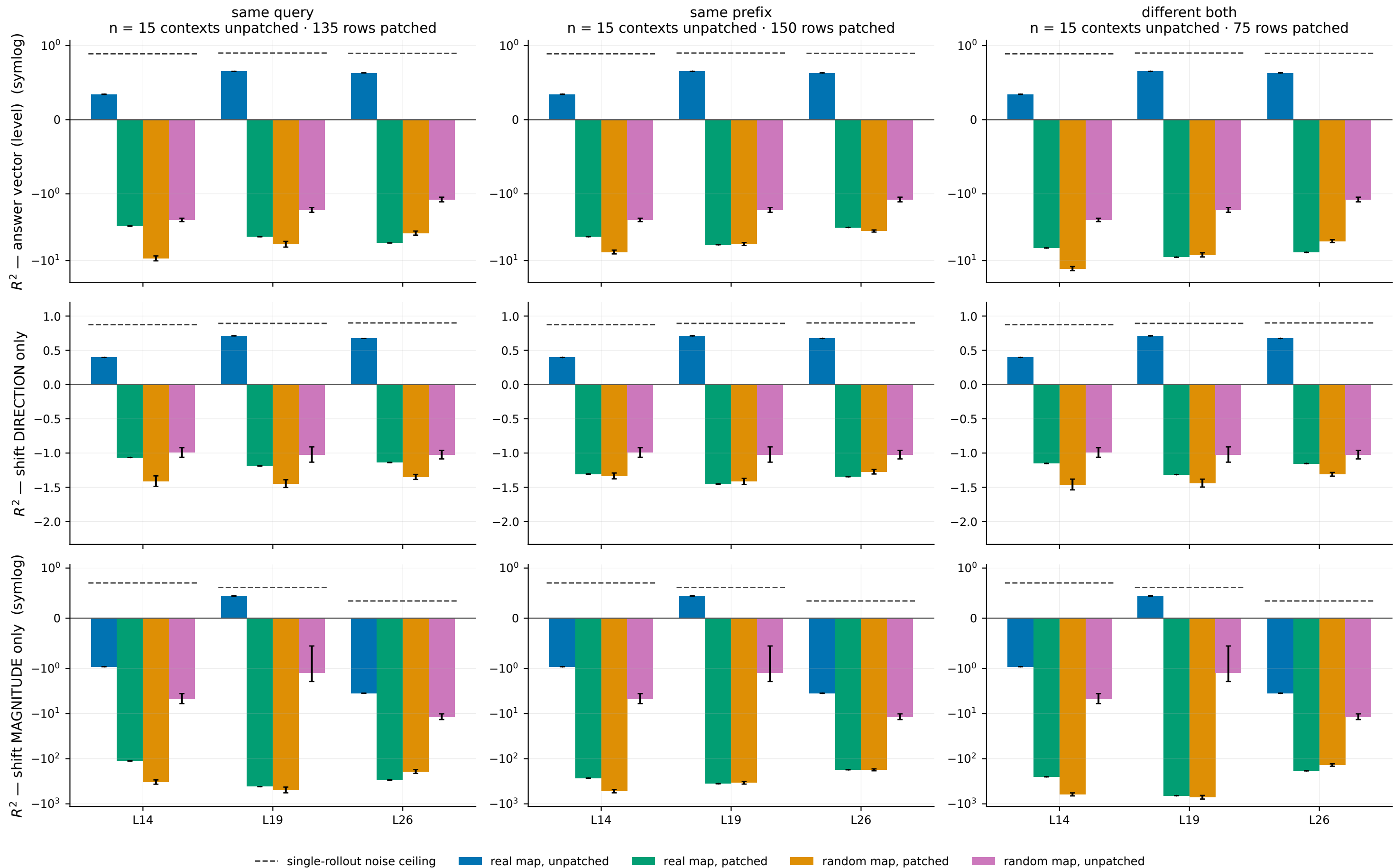
Banked-map R^2 at the context-end v_C : real vs spectrum-matched random map, unpatched vs patched
