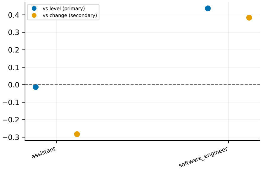
sycophancy: rho vs LEVEL (primary) vs rho vs change (secondary)
