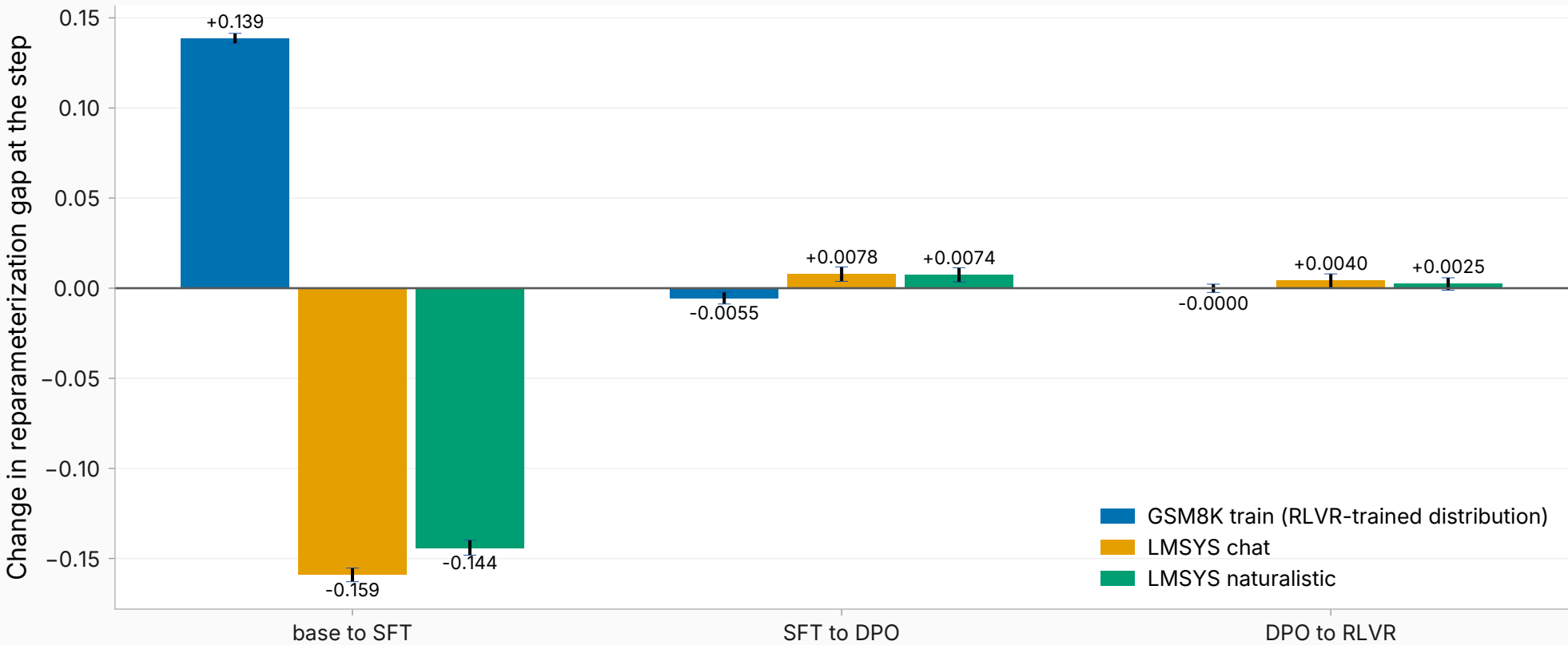
Adjacent-stage gap increments (recalibrated scale, layer 30)
