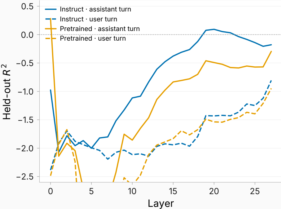
Two-turn track: map strength by layer, assistant vs user turn
