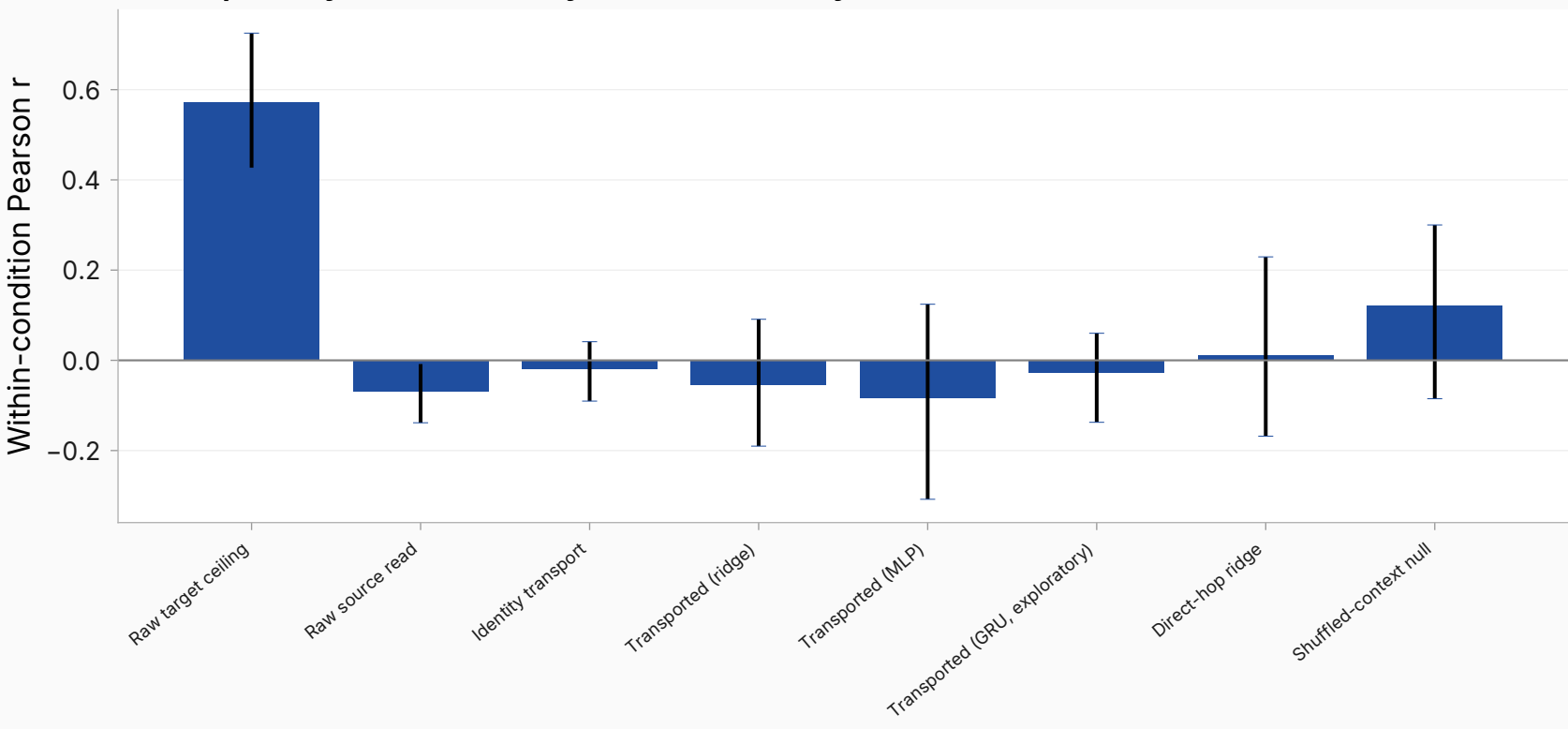
evil — primary \ell^*=20 — many_shot (source layer 0)
