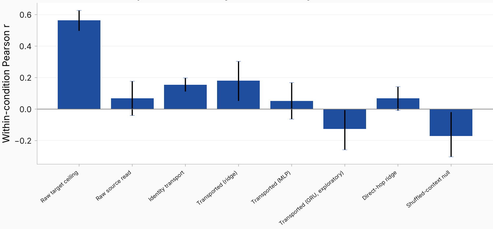
hallucination — companion \ell^*=24 — system (source layer 0)
