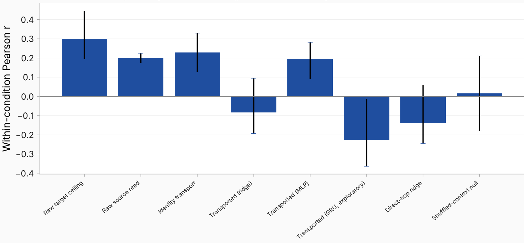
hallucination — primary \ell^*=17 — many_shot (source layer 0)
