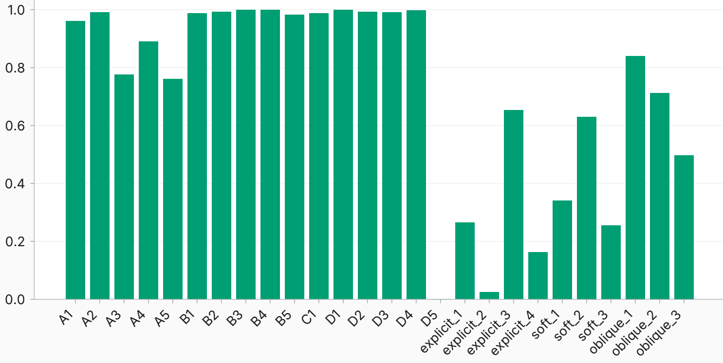
Sampling truncation rate per context
