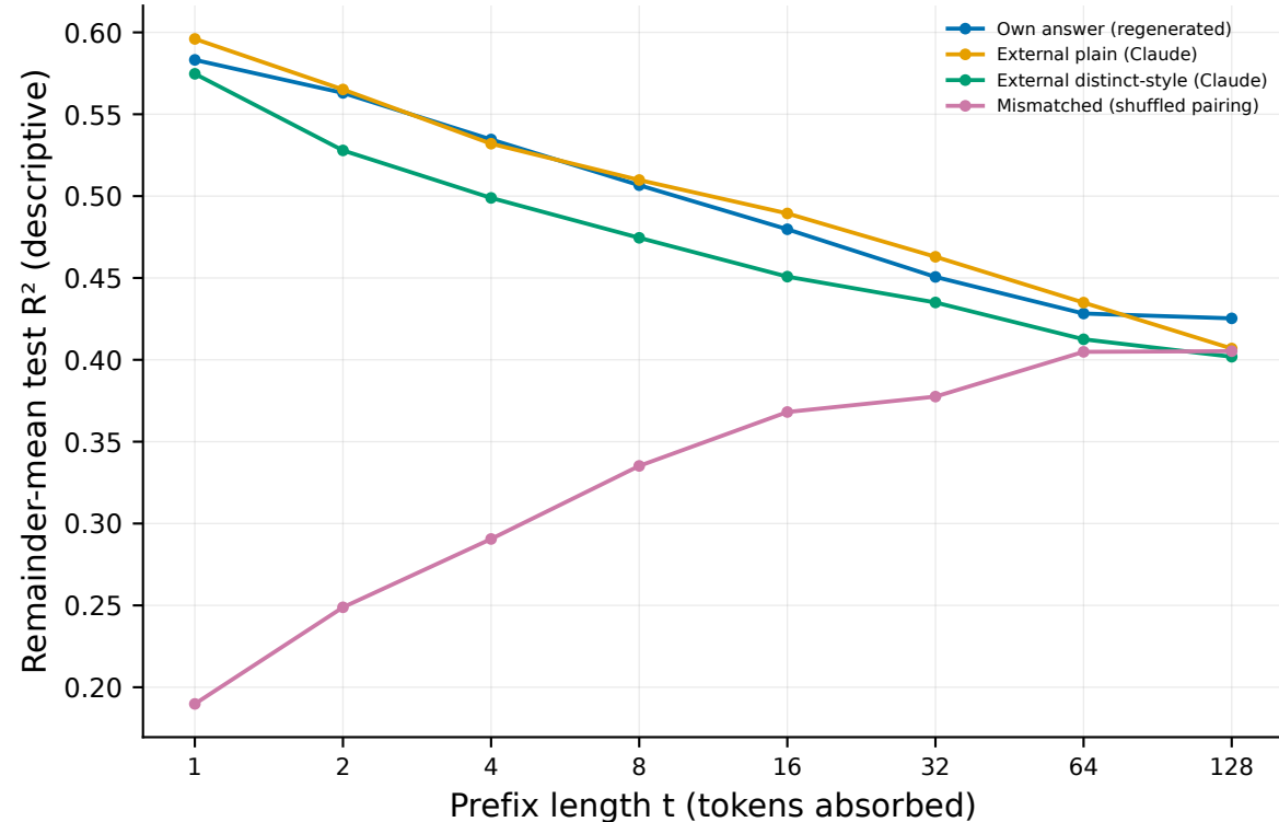
Prediction of the remainder as the prefix is absorbed Descriptive view; survivor populations vary per t
