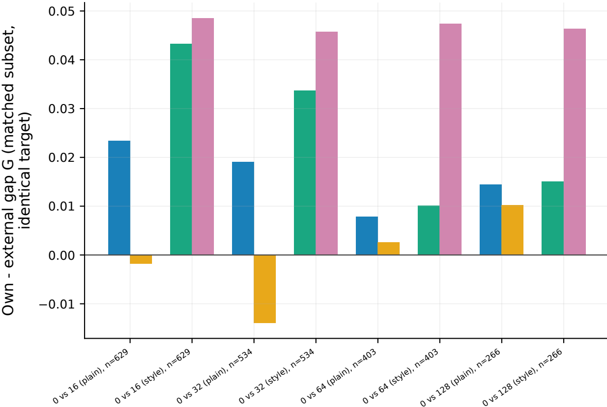
Does absorbing the answer prefix close the own-advantage? Left bar: G at t=0 ; right bar: G at t (layer 20, common survivors, identical target)
