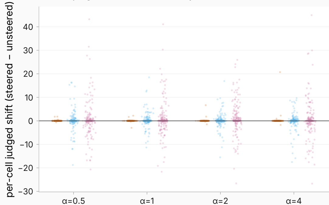
Per-cell judged shifts (200 contexts per stratum)
