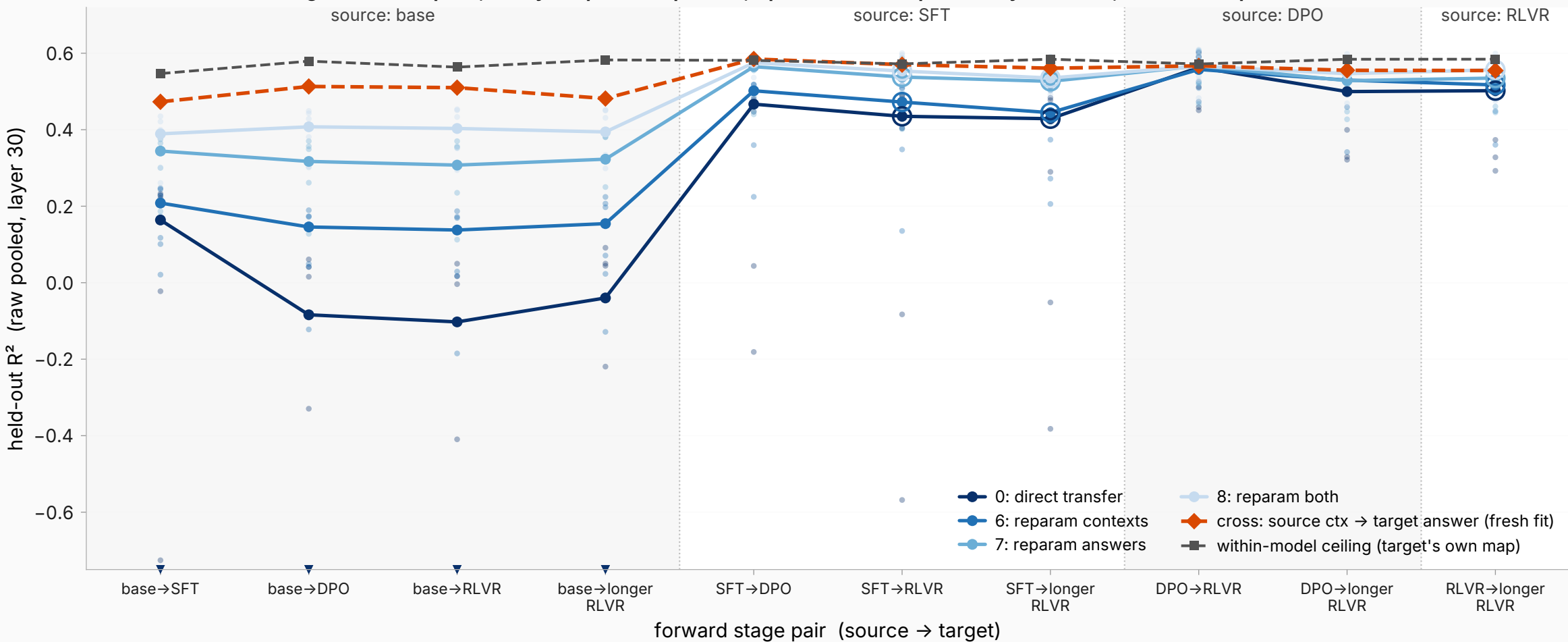
Every forward pair of the Tülu-3 ladder: how much of the context→answer map survives median over 7 non-degenerate corpora, every corpus overplotted; open markers = point-only (round B, no bootstrap draws)
