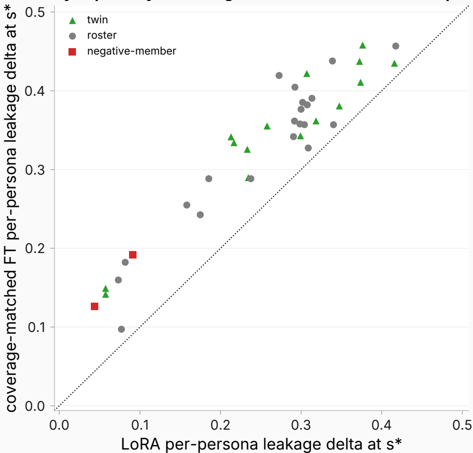
sycophancy: coverage-matched FT vs LoRA (Spearman \rho = 0.89 )
