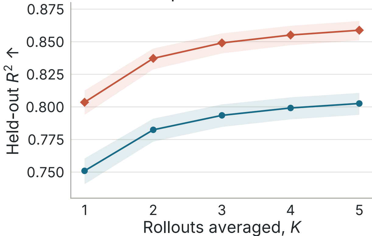
Variance explained
