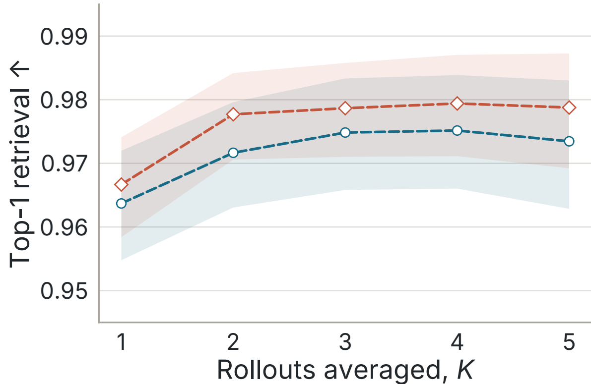
Answer identification
