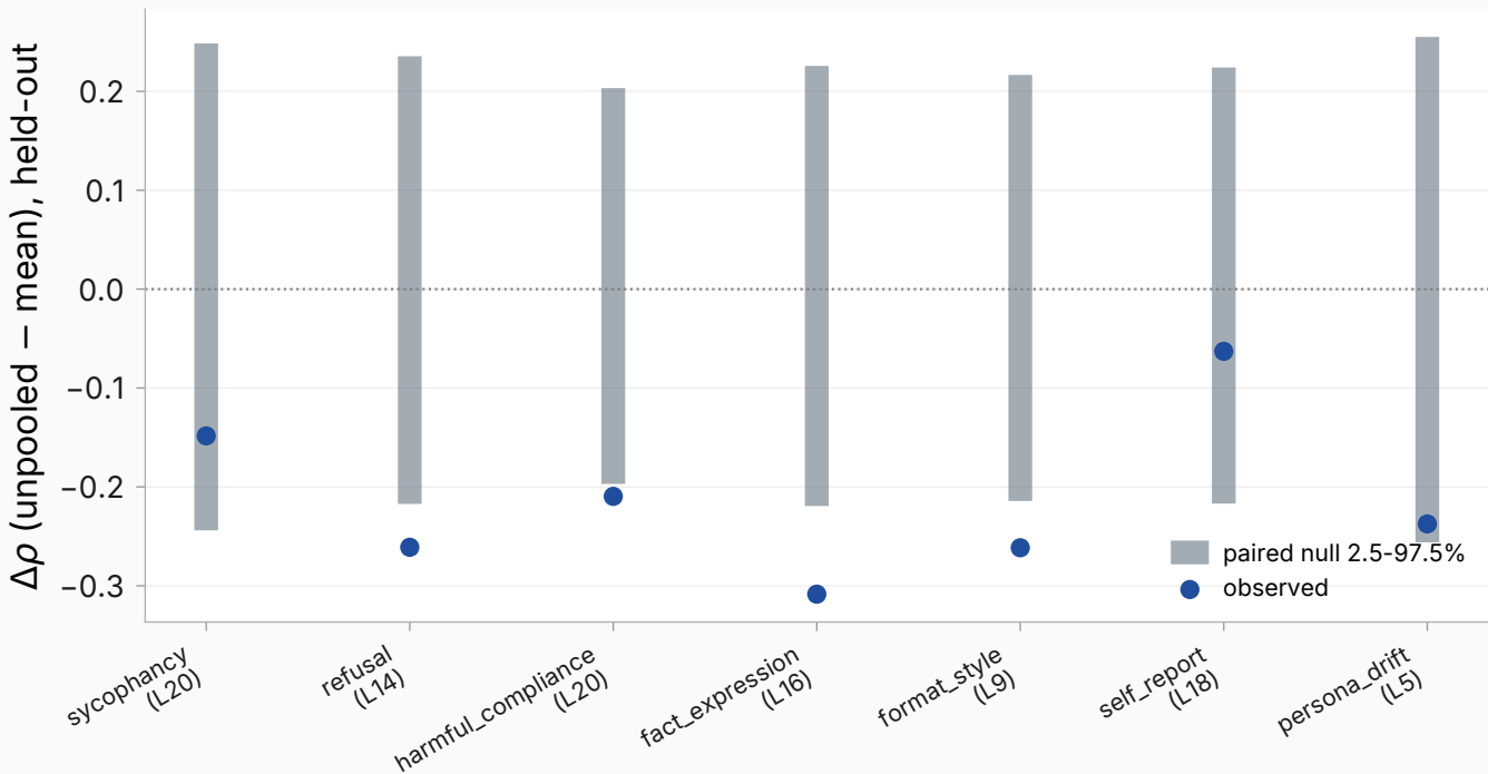
Fixed best-mean-layer paired unpooled-vs-mean contrast
