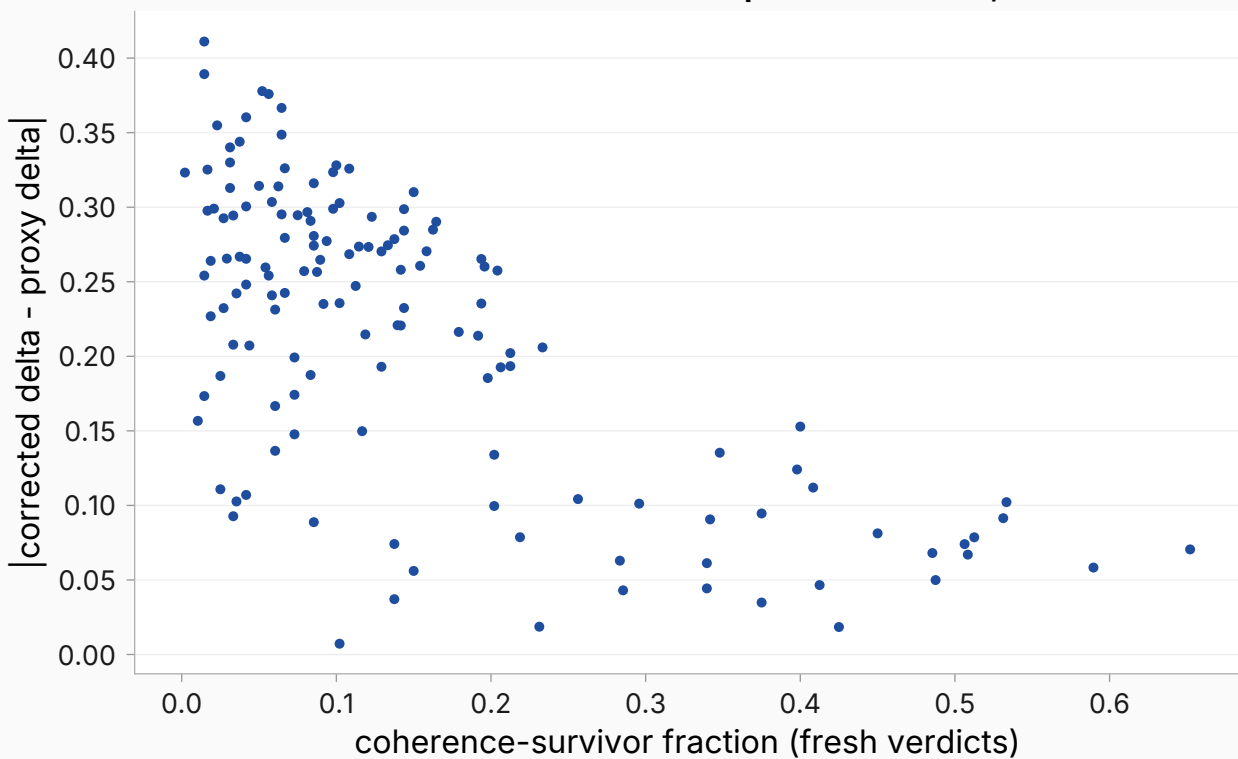
Delta shift vs survivor fraction (manipulation check, not a discovery)
