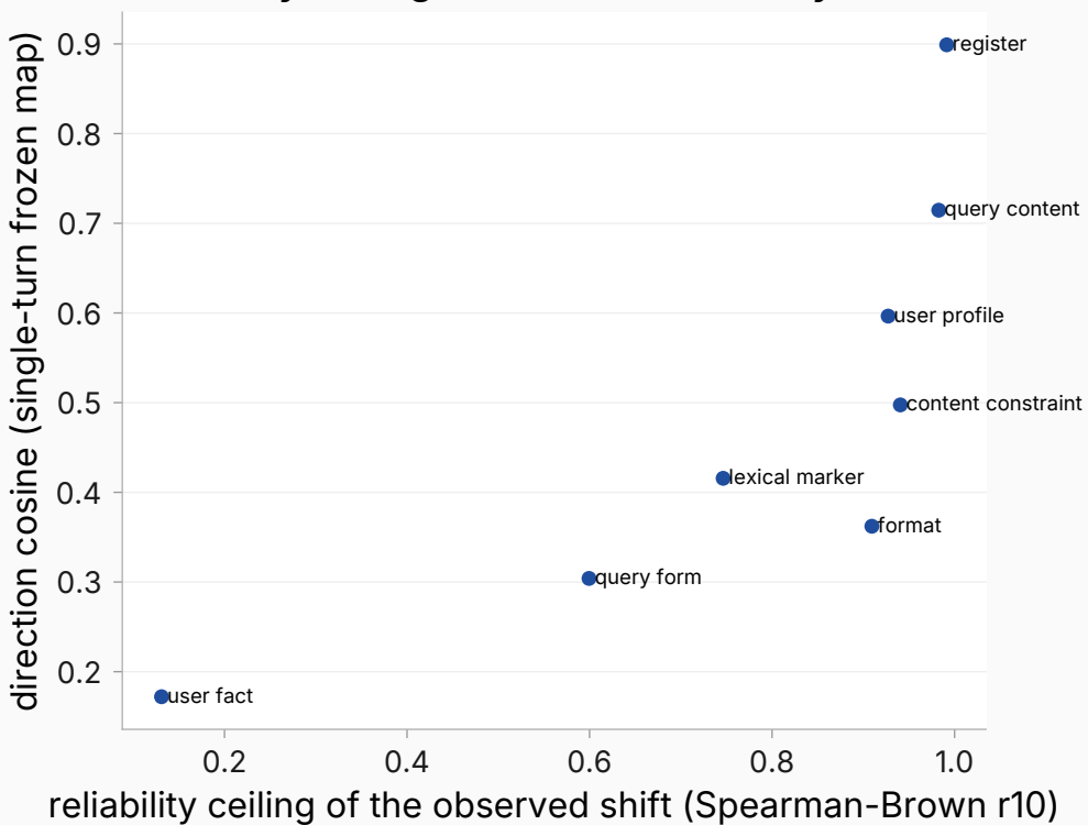
Reliability ceiling vs direction recovery
