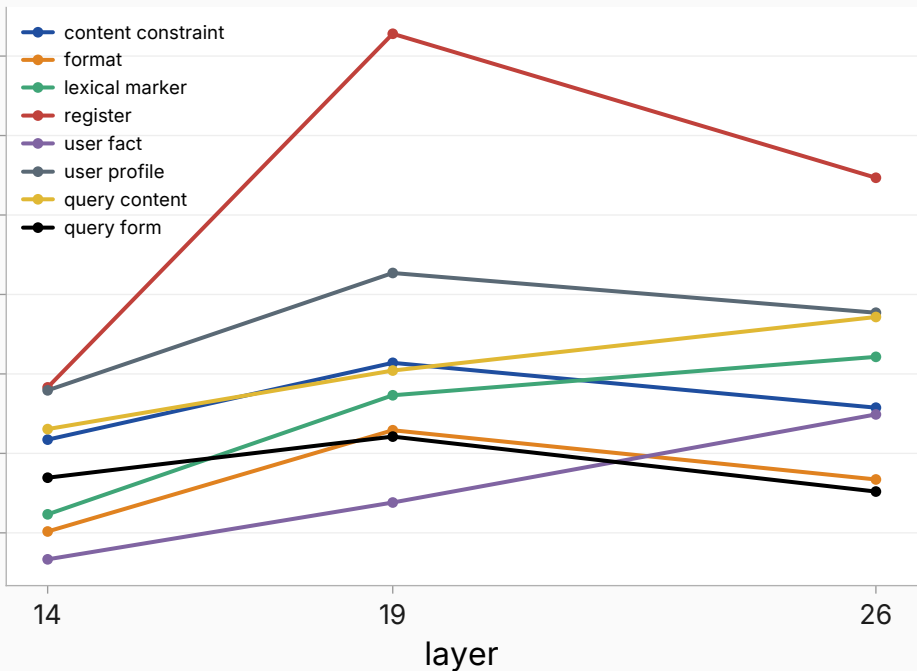
Layer sensitivity (identity baseline only)
