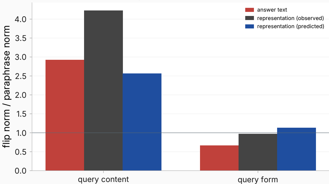
Query axes: text vs representation dissociation
