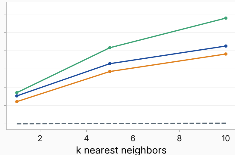
euclidean distance
