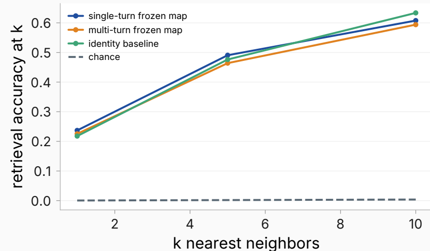
cosine distance
