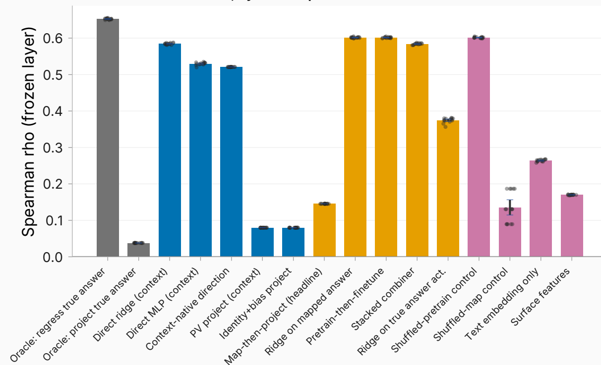
sycophancy, pooled-natural direction
