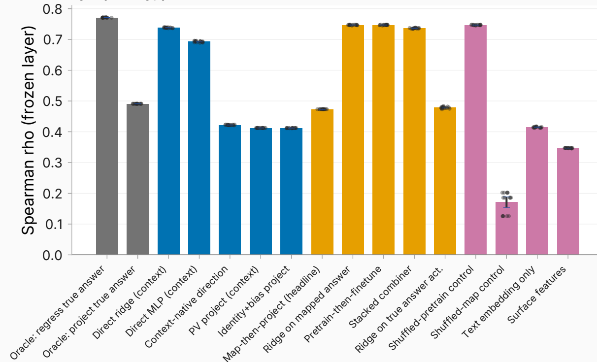
sycophancy, pooled-natural direction
