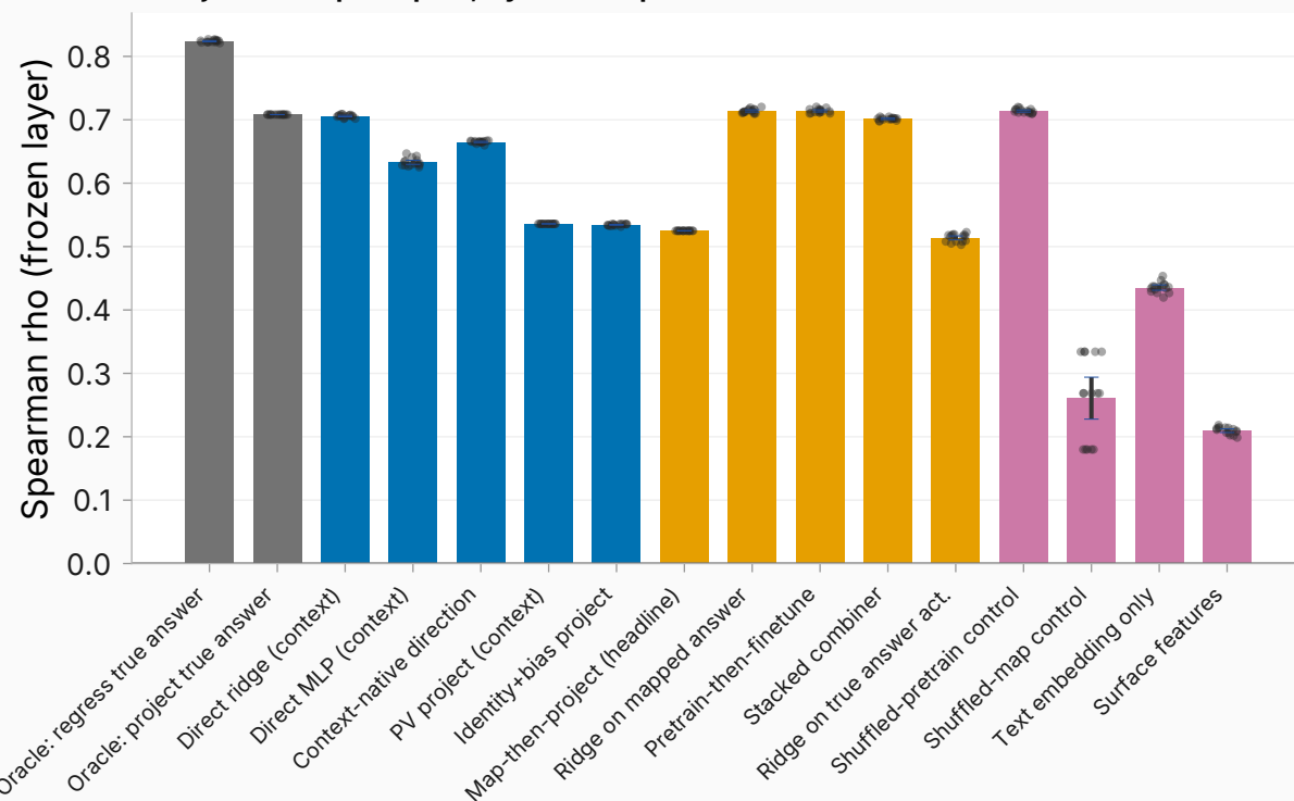
sycophancy (Reddit advice), synthetic-pair direction
