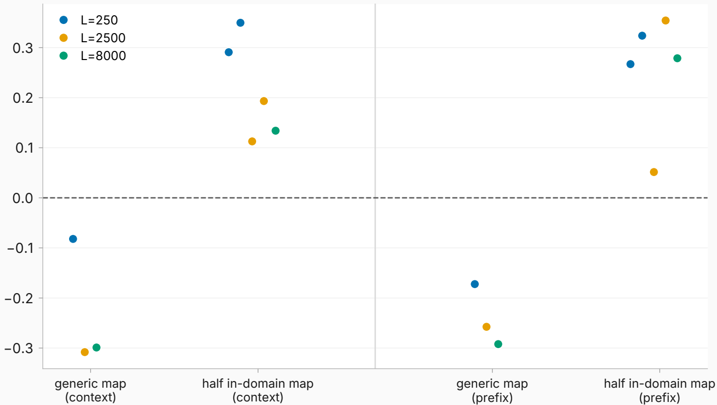
Evil composition cells: fitting the map on half in-domain contexts flips its sign (each dot = one cell, single draw and seed — preliminary)
