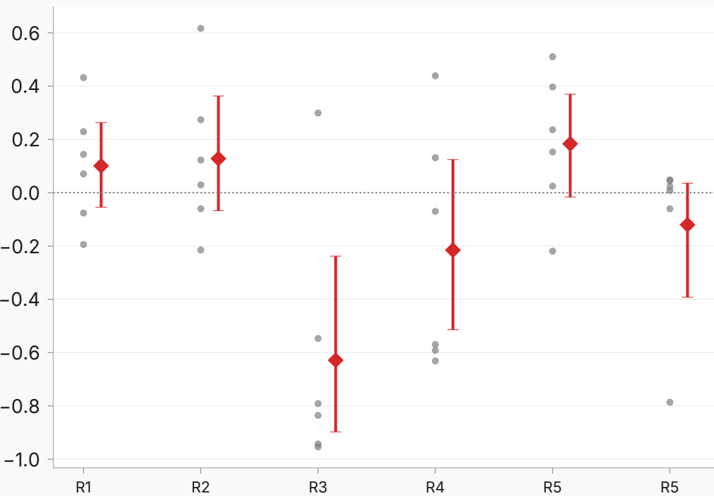
context-end
