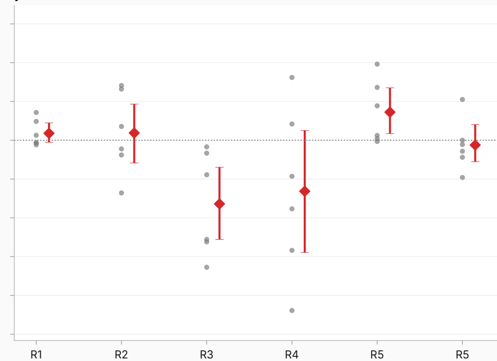
prefix-end
