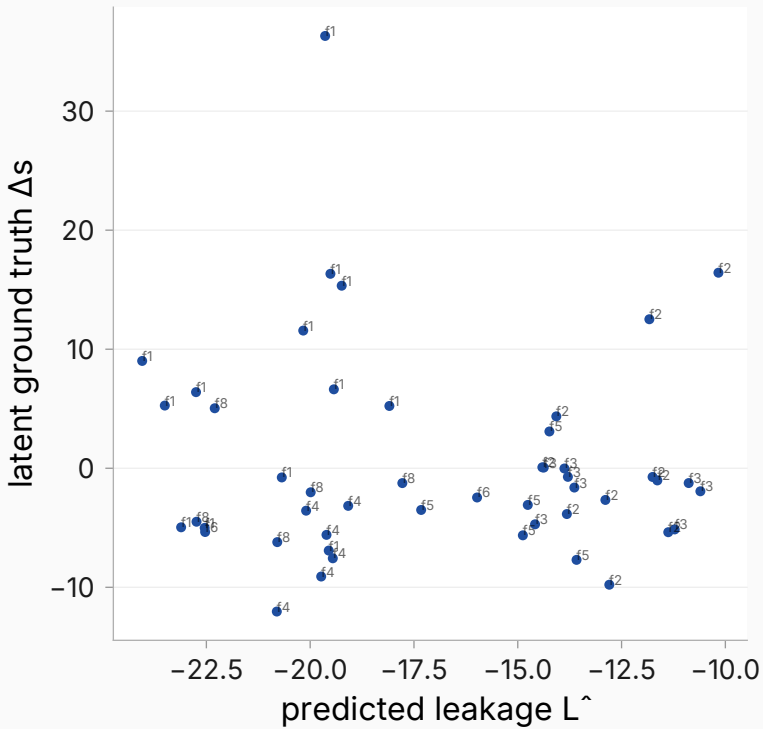
ic_librarian_contra_d2_seed42 (p=0.025)
