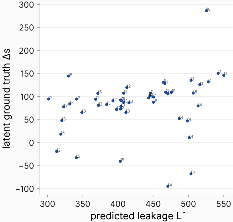
tf_rev_librarian_contra_d1_seed42 ( \rho=0.407 )
