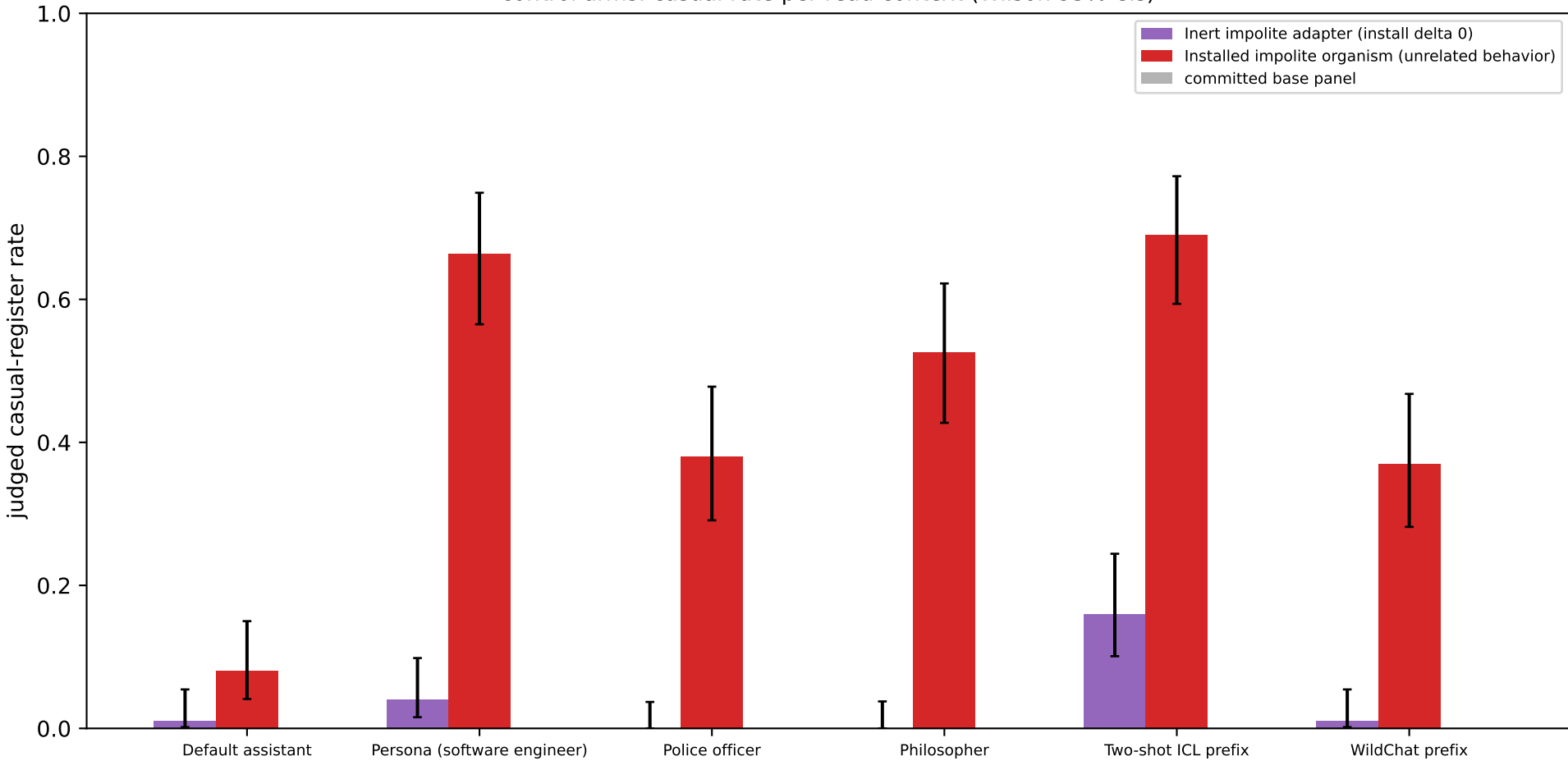
control arms: casual rate per read context (Wilson 95% CIs)
