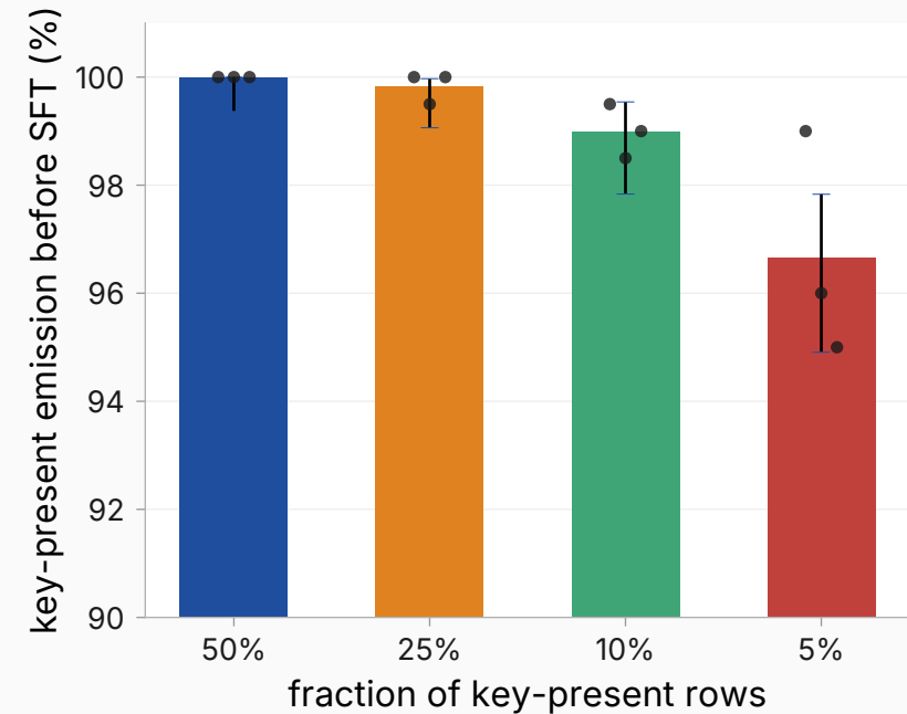
Before SFT: rarer positives sharpen the key-gate but install slightly weaker at 5%
