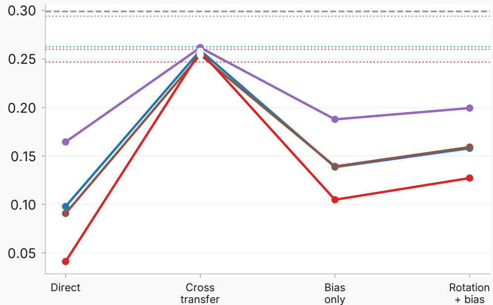
inserted — base
