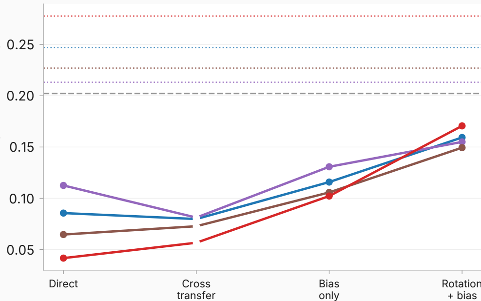
on-policy — base
